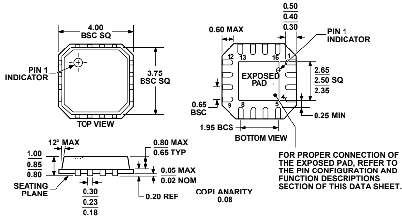
Figure 54. 16-Lead Lead Frame Chip Scale Package [LFCSP_VQ] 4 mm × 4 mm Body, Very Thin Quad (CP-16-13)
