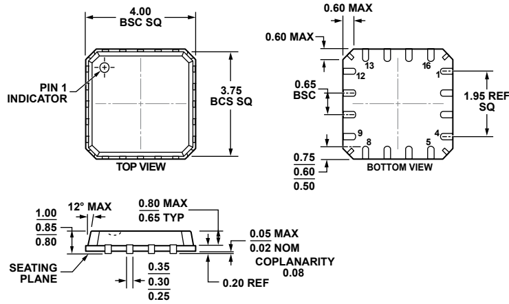
Figure 55. 16-Lead Lead Frame Chip Scale Package [LFCSP_VQ] 4 mm × 4 mm Body, Very Thin Quad, with Hidden Paddle CP-16-19
